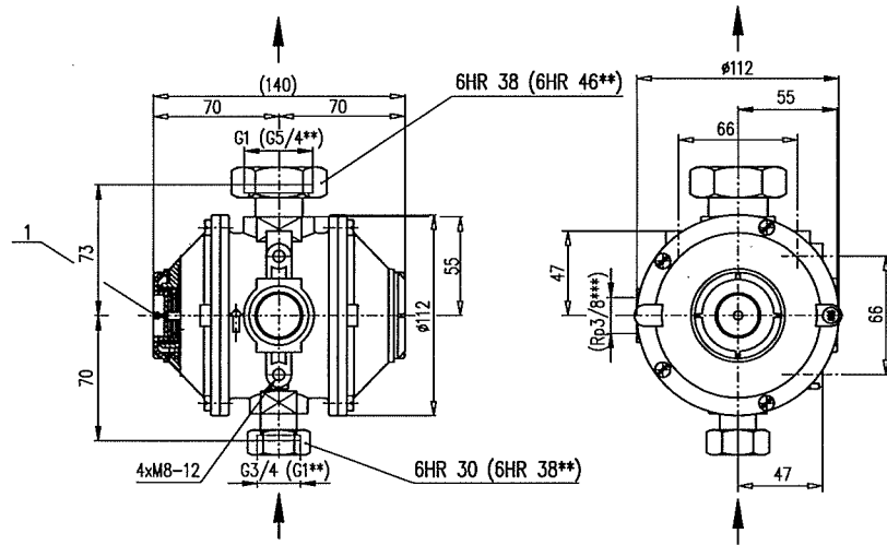
RTP..-M..-P with axial ( direct ) position of inlet/outlet connection and coupling nuts
