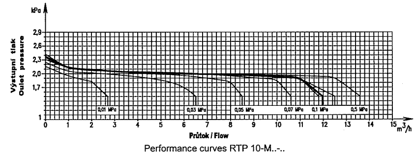
Performance curves RTP 10-M..-
