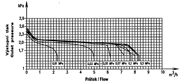
Performance curves RTP 6-M..-
