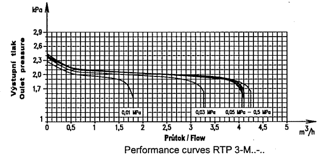
Performance curves RTP 3-M..-
