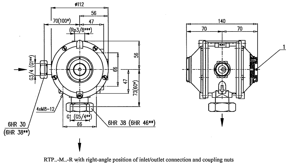
RTP..-M..-R with right-angle position of inlet/outlet connection and coupling nuts
